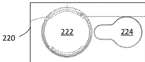
Top view of bayonet interface (phone side)
