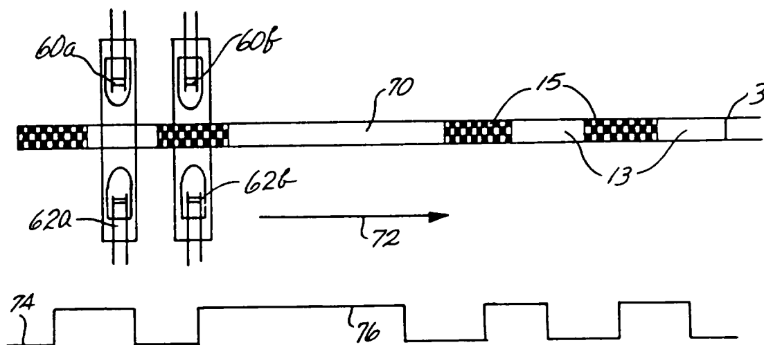
Fig. 6c (PRIOR ART)
