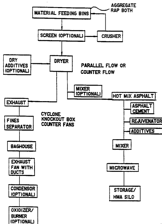
SYSTEM CONFIGURATION FOR HOT MIX ASPHALT PLANT
