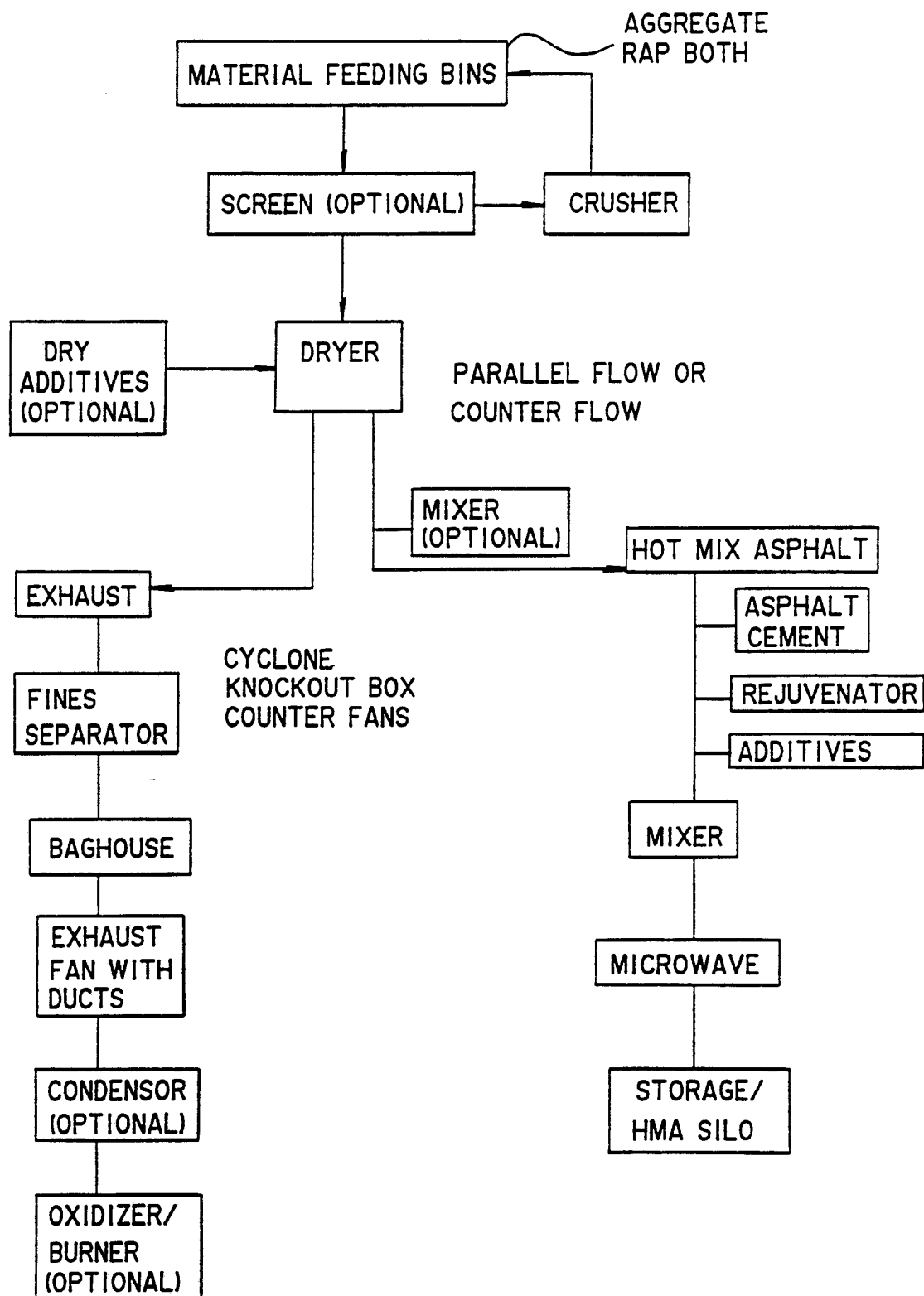
SYSTEM CONFIGURATION FOR HOT MIX ASPHALT PLANT
