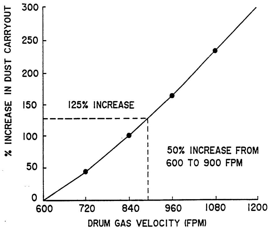
DUST CARRYOUT VS. DRUM GAS VELOCITY
