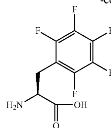
Phe(pentaF)
