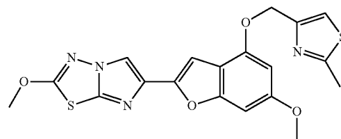
1A. (2-Methylthiazol-4-yl)methanol
