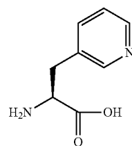
3-Pya
