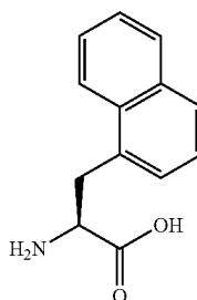
1-Naphthyl-Ala
