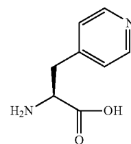
4-Pya
