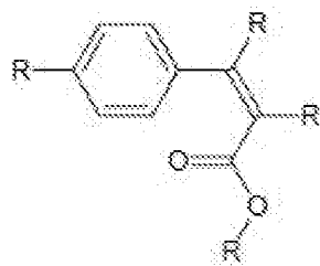
Cinnamate derivatives
