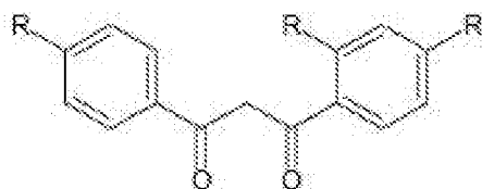
Dibenzoyl methane derivatives
