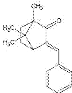
Camphor derivatives
