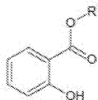
Salicylate derivatives
