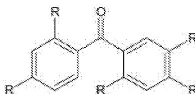
Benzophenone derivatives
