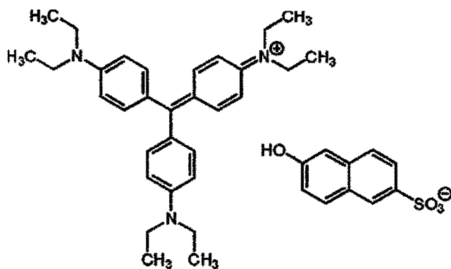
Ethyl violet
