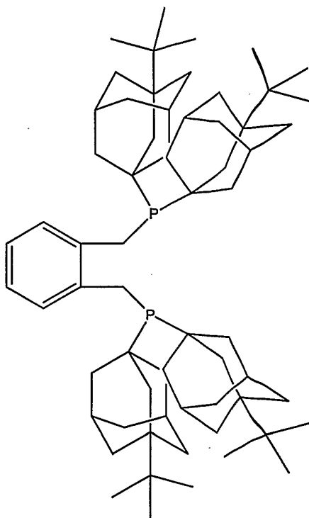
1,2-bis(di-1-(5-tert-butyladamantyl) phosphinomethyl) benzene
