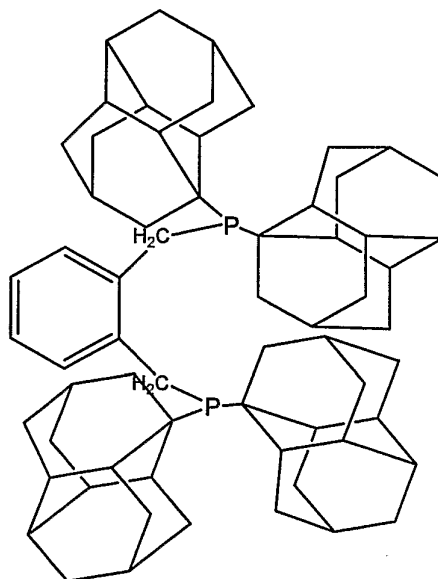
1,2 bis(di-congressylphosphinomethyl) benzene
