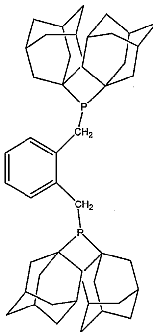
1,2 bis(diadamantylphosphinomethyl) benzene
