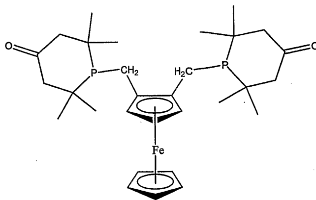
1,2-bis-, -(P-(2,2,6,6,-tetramethylphosphinan-4-one))dimethylferrocene
