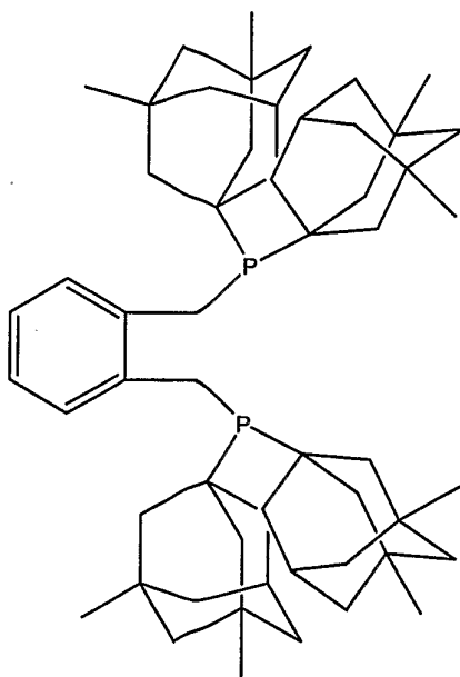
1,2-bis(di-1-(3,5-dimethyladamantyl) phosphinomethyl) benzene
