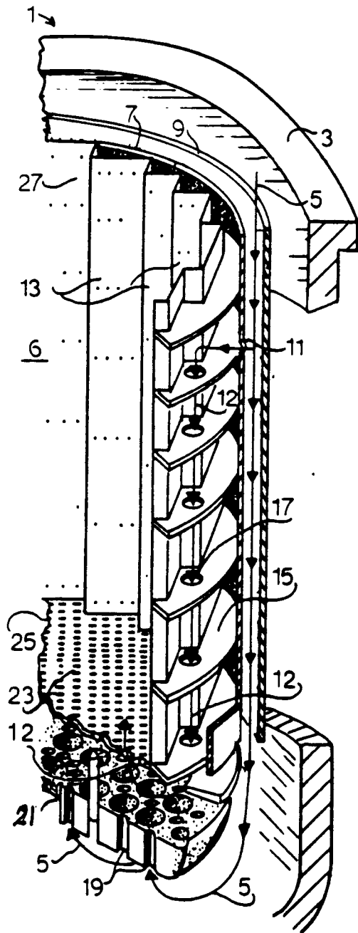
FIG. 1 - PRIOR ART
