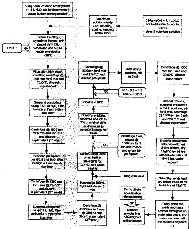
Figure 2 Pharmaceutical-Grade Ferric Citrate manufacture Flow Chart
