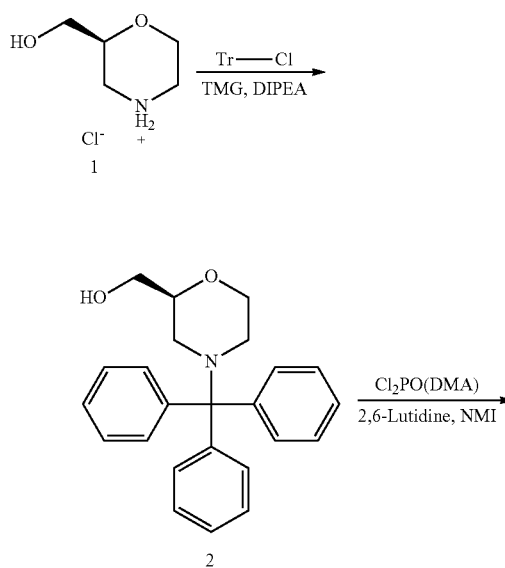
Reaction Scheme 2. Preparation of Activated Morpholino Abasic Subunit
