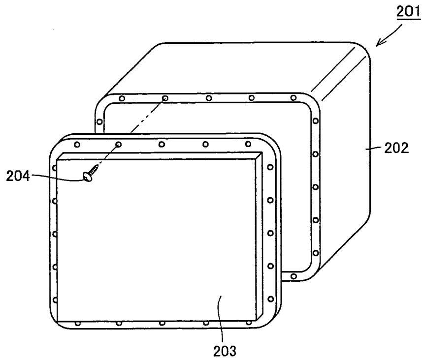
FIG.22 PRIOR ART
