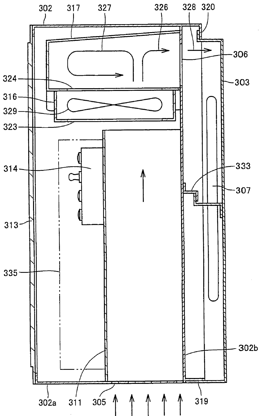
FIG.26 PRIOR ART
