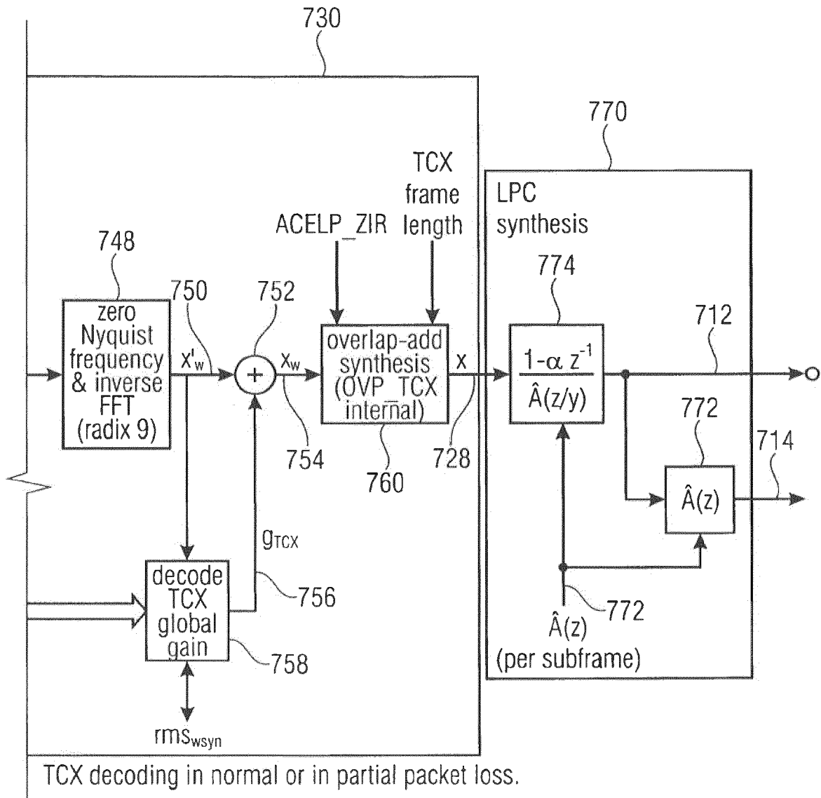
Block diagram of the TCX decoder
