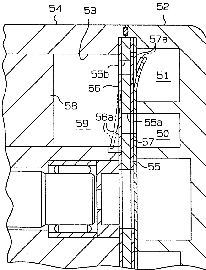
Fig. 17 Prior Art
