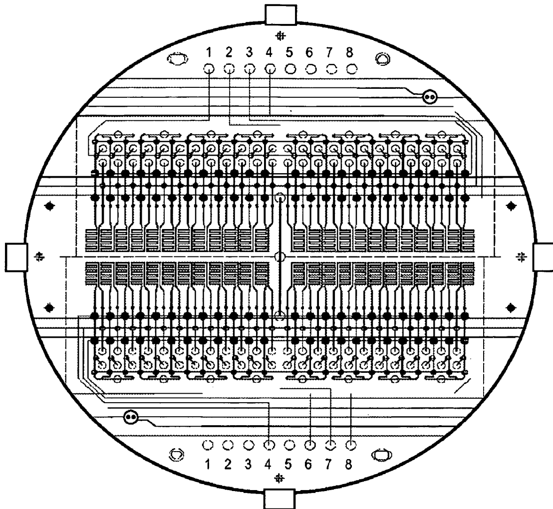
Fabrication chip with 2 Microfluidic Chip Devices Actual chip on 4 inch diameter circle Standard 9mm center to center spacing for compatibility with lab
