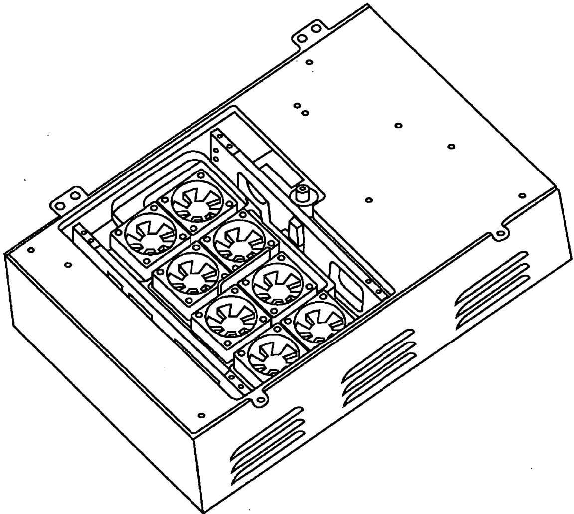
Thermal control element: bottom view
