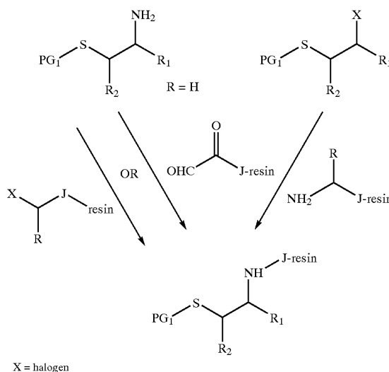
Scheme I Solid-phase synthesis of ECL auxiliary derivatized molecules
