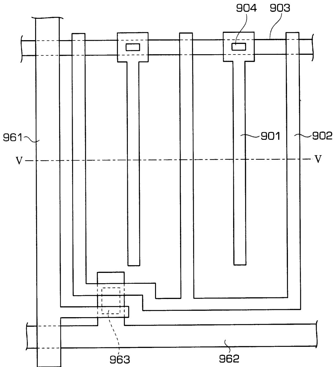
FIG. 4 PRIOR ART
