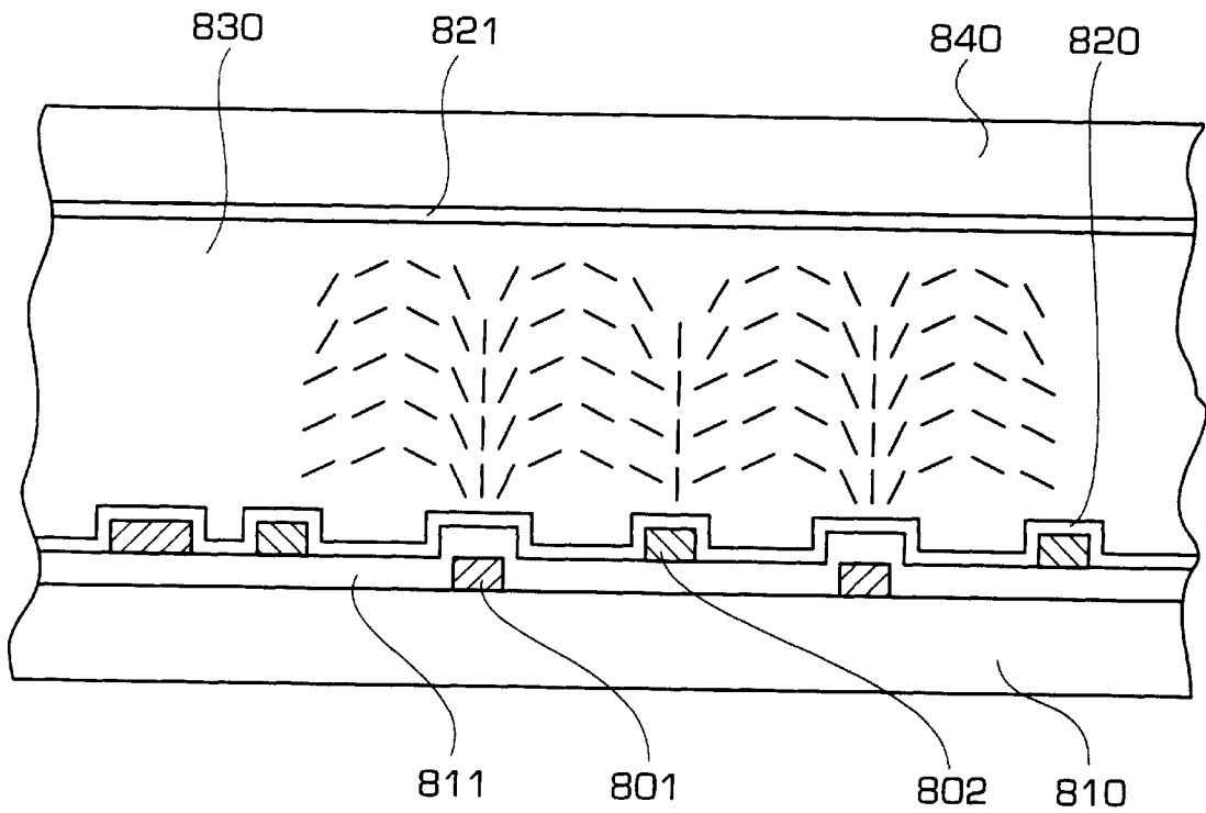
FIG. 3 PRIOR ART
