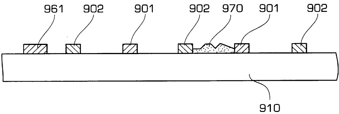
FIG. 6 PRIOR ART
