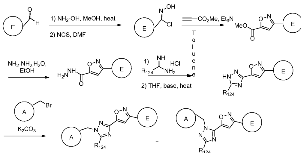
Scheme 16a
