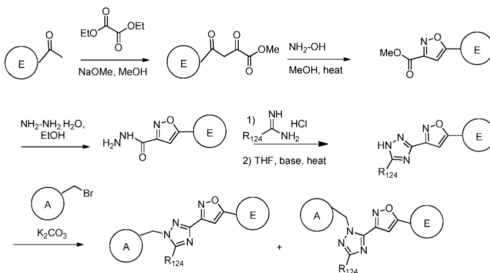
Scheme 16b
