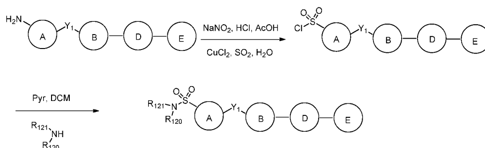
SCHEME 11:
