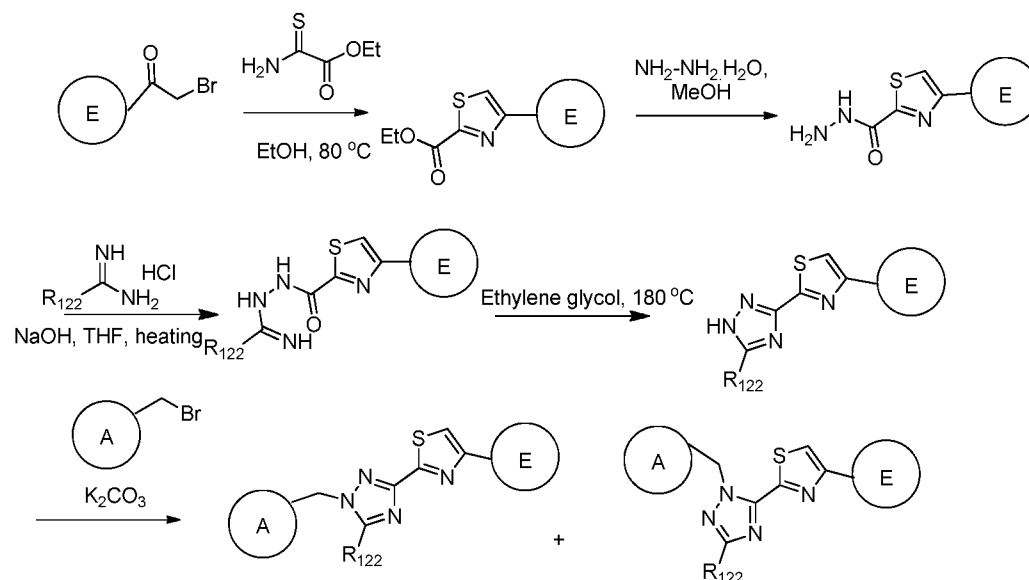
SCHEME 14:
