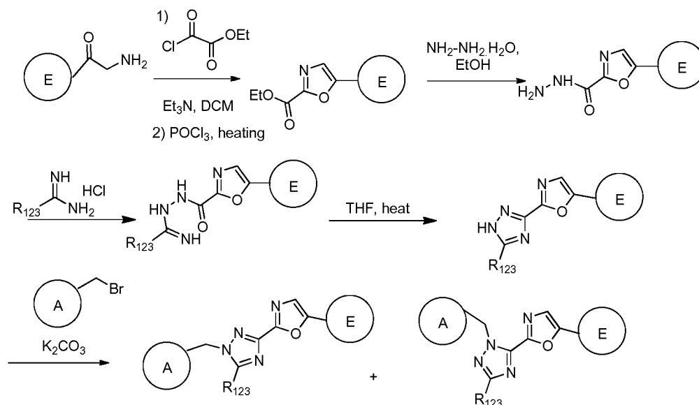
SCHEME 15:
