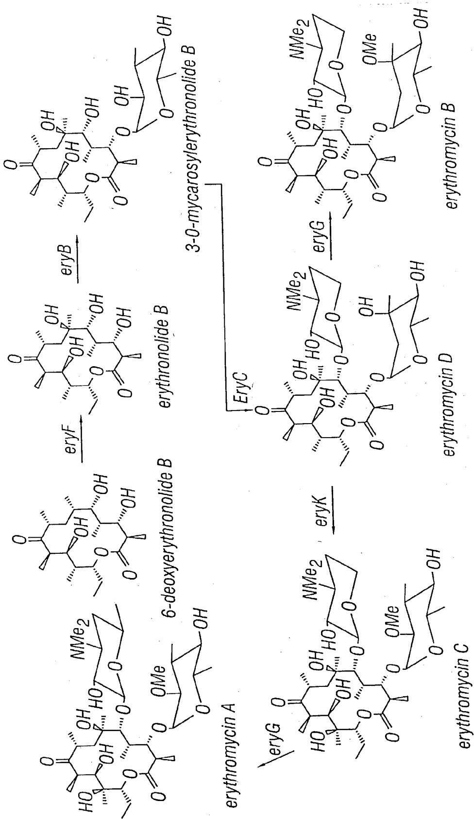
Post-PKS Biosynthesis of Erythromycins
