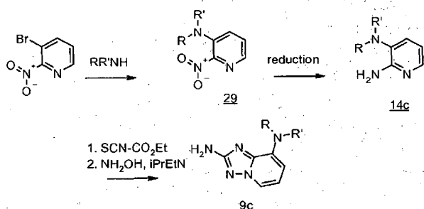
Scheme 10
