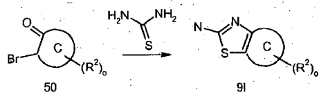
Scheme 16
