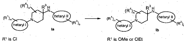
Scheme 29
