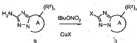
Scheme 17
