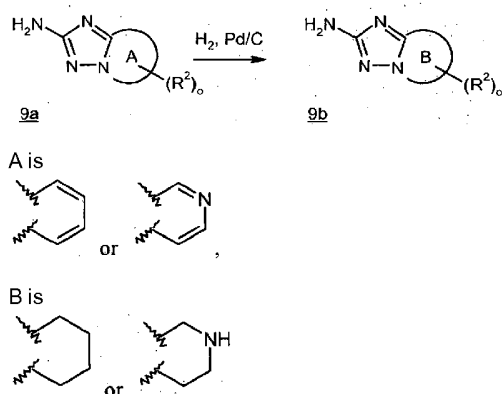
Scheme 9
