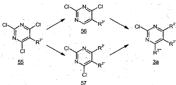
Scheme 19
