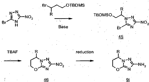
Scheme 14
