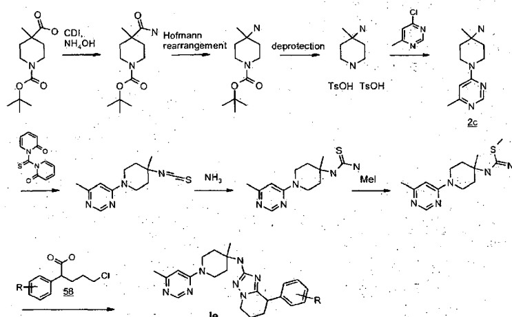
Scheme 32
