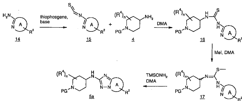
Scheme 5
