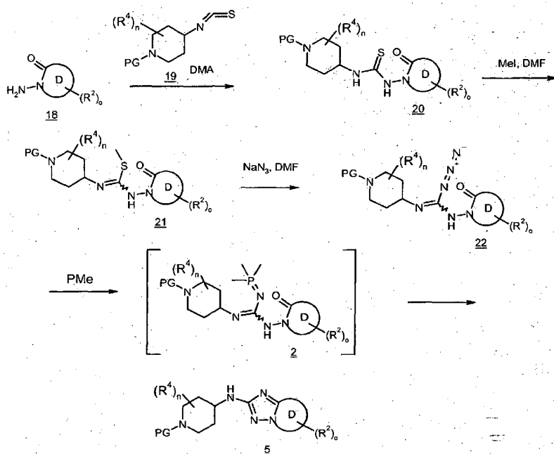
Scheme 6
