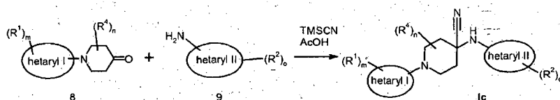
Scheme 30
