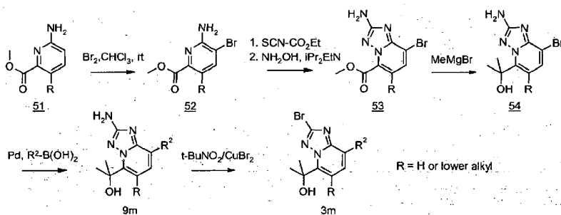
Scheme 18
