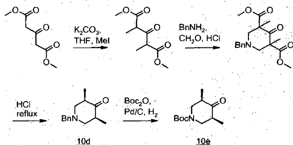
Scheme 21
