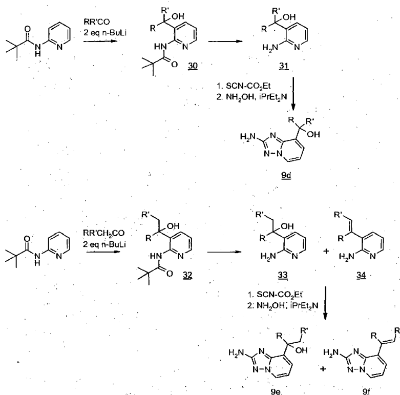
Scheme 11
