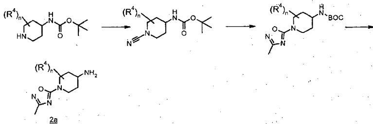
Scheme 25
