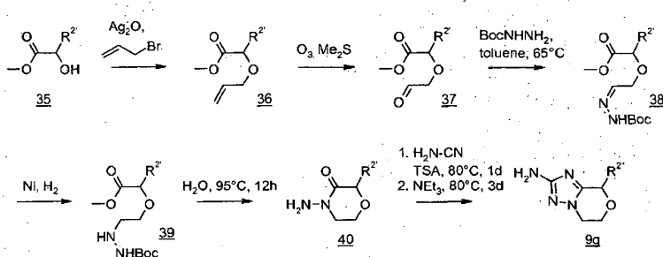
Scheme 12
