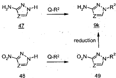
Scheme 15
