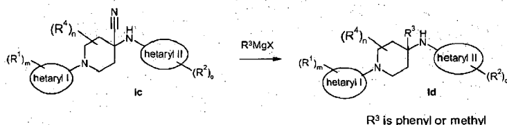
Scheme 31
