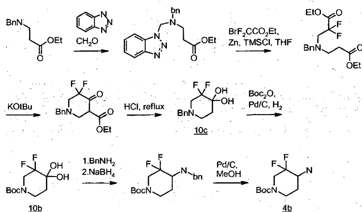
Scheme 28
