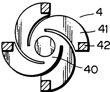
FIG. 8 PRIOR ART
