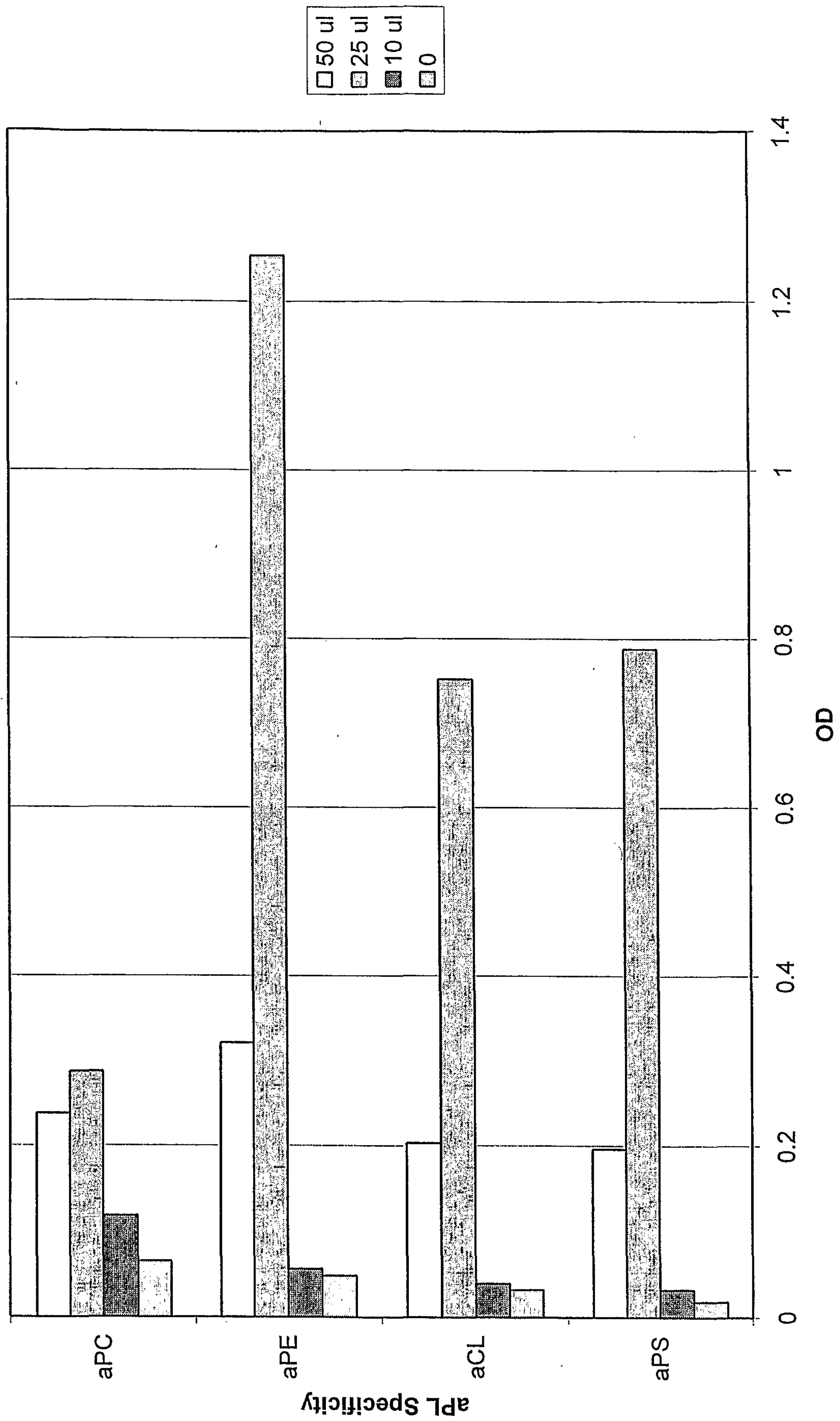
Figure 23 Hemin Dose Response
