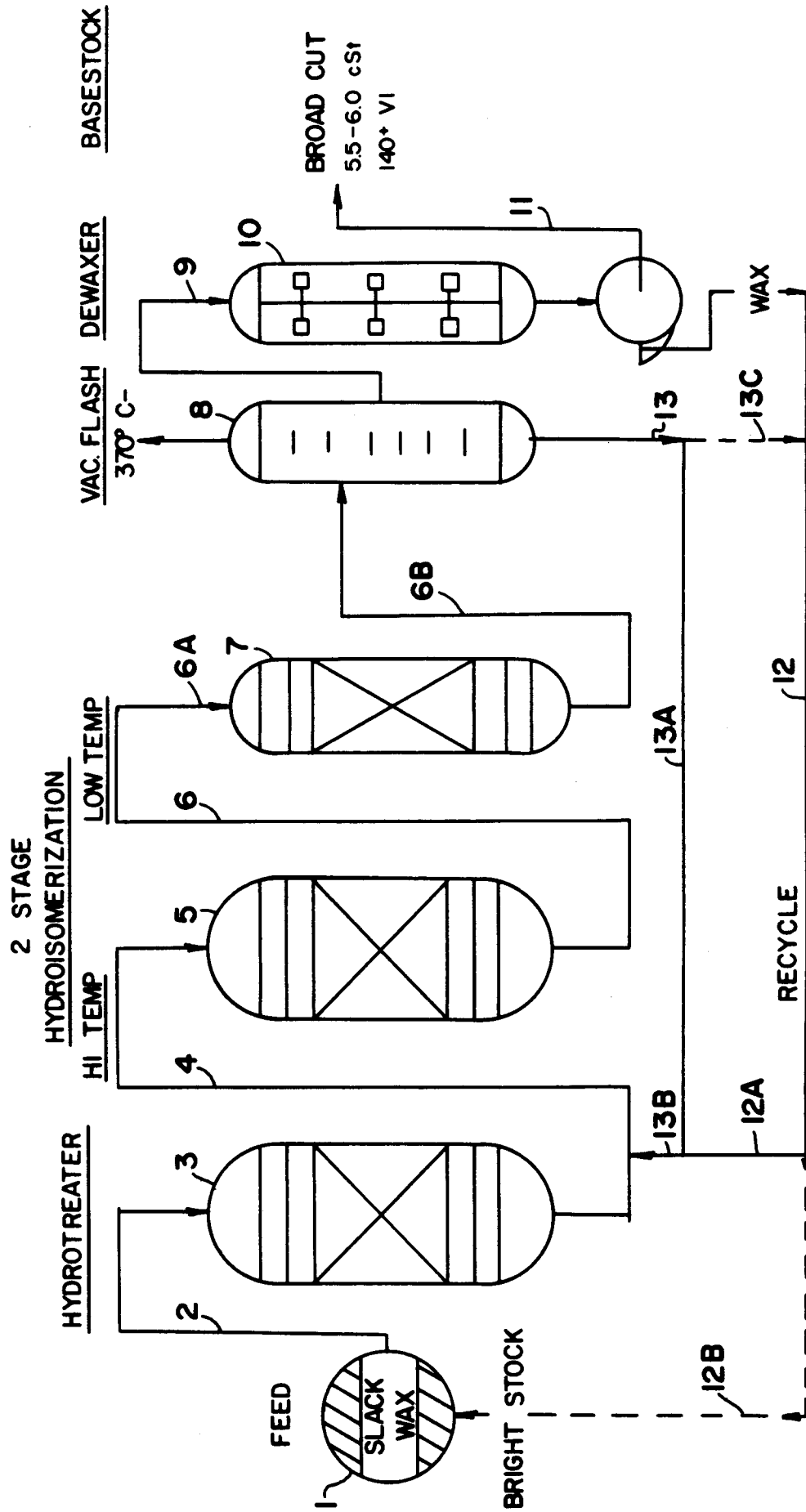
FIG. 2 SLACK WAX ISOMERIZATION PROCESS
