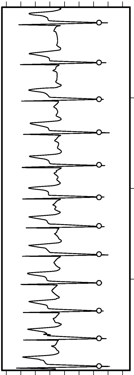
NSR Strip
