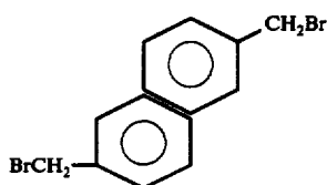
4,4'-Bis(bromomethyl) diphenyl methane
