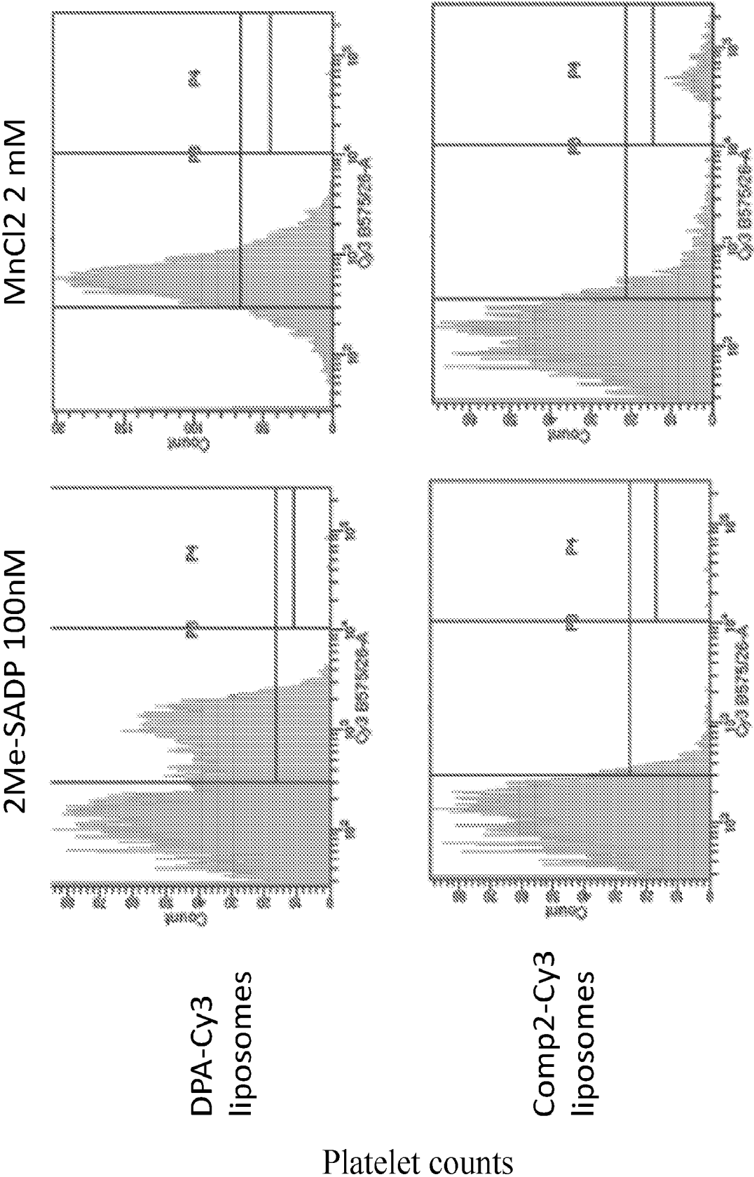
Cy3 (liposome binding) Figure 1 (continued)
