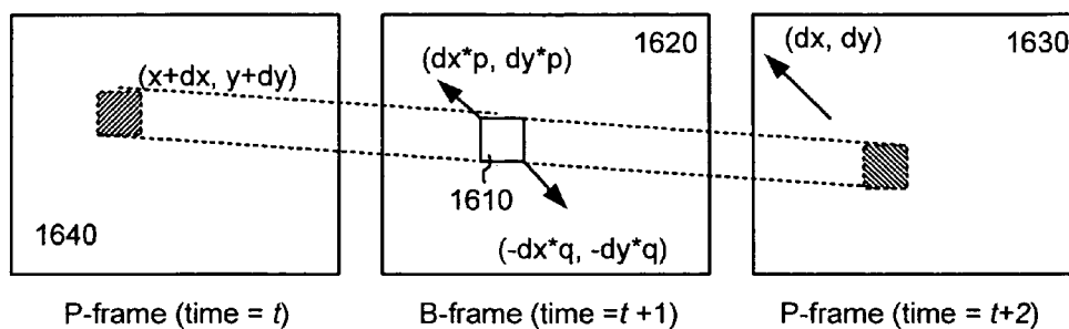
Figure 16, prior art
