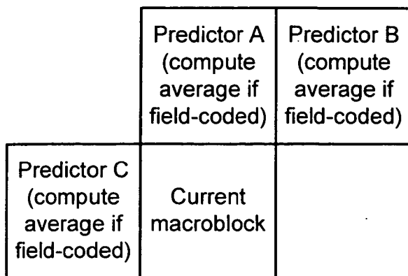
Figure 11, prior art
