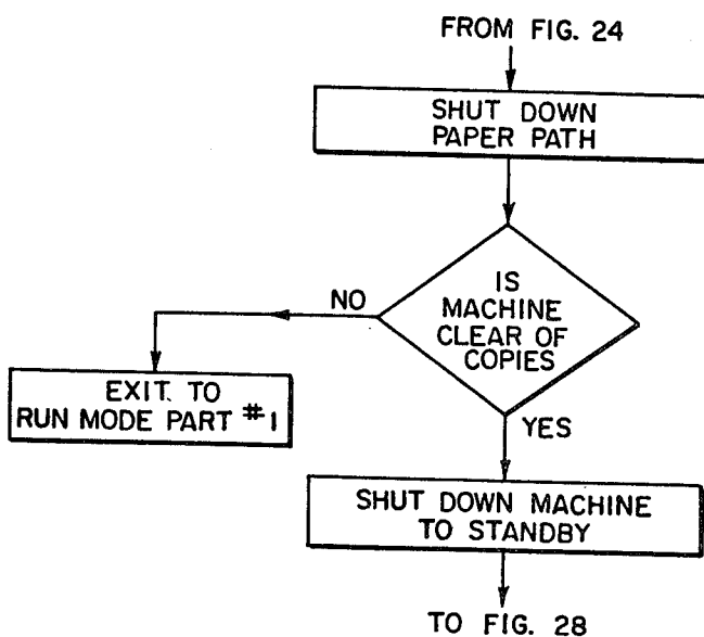
CYCLE OUT FIG. 27
