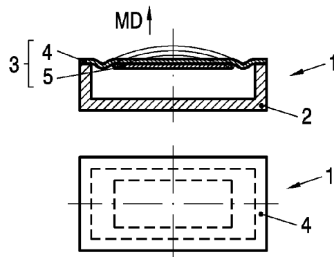
Fig. 4 (Prior Art)
