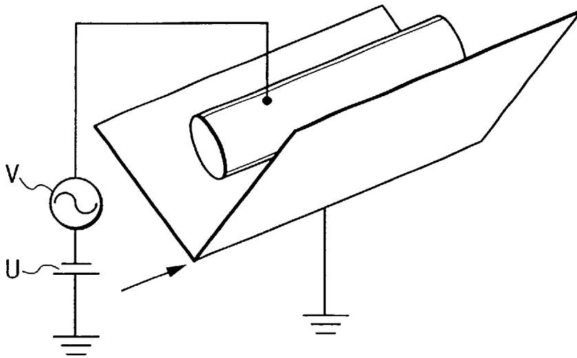
MONOPOLE ELECTRODE
