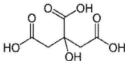
Citric acid (un-neutralized)
