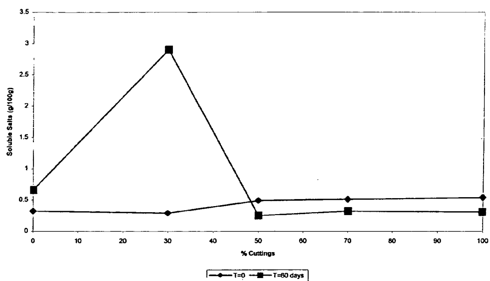
Fig.13 Soluble Salts Concentration – Second Test
