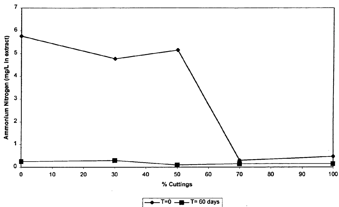
Fig.14 Ammonium Nitrogen Concentration – Second Test
