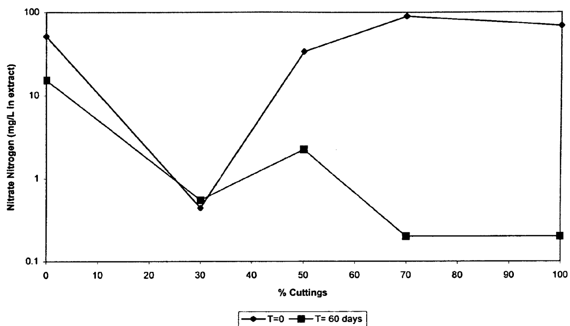
Fig.15 Nitrate Nitrogen Concentration – Second Test
