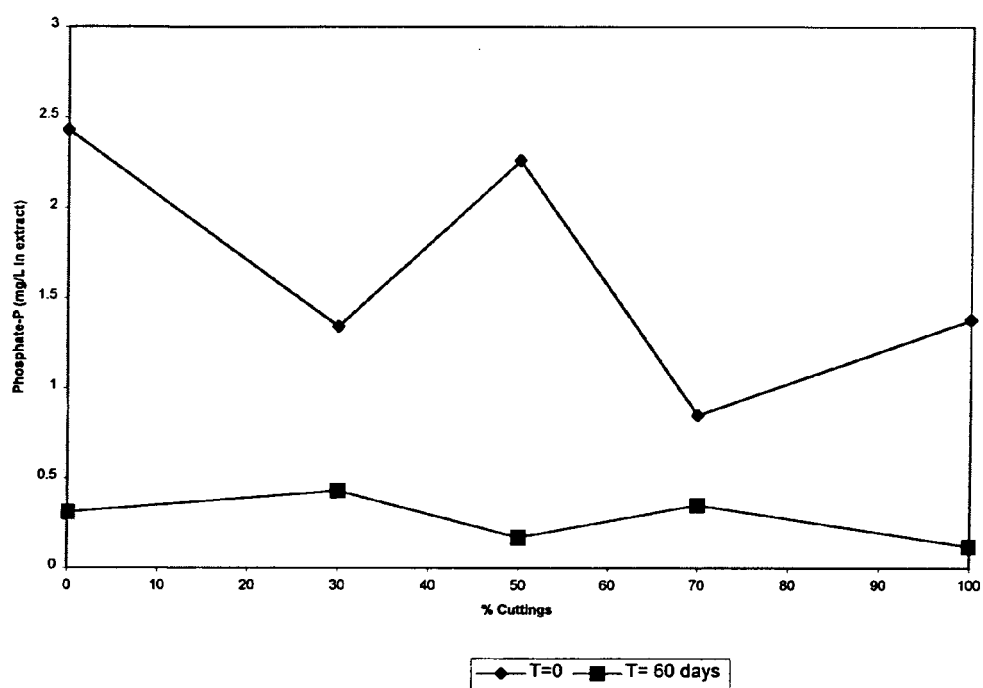
Fig.17 Phosphate Phosphorous Concentration – Second Test
