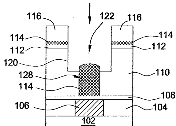
FIG. 1C (PRIOR ART)
