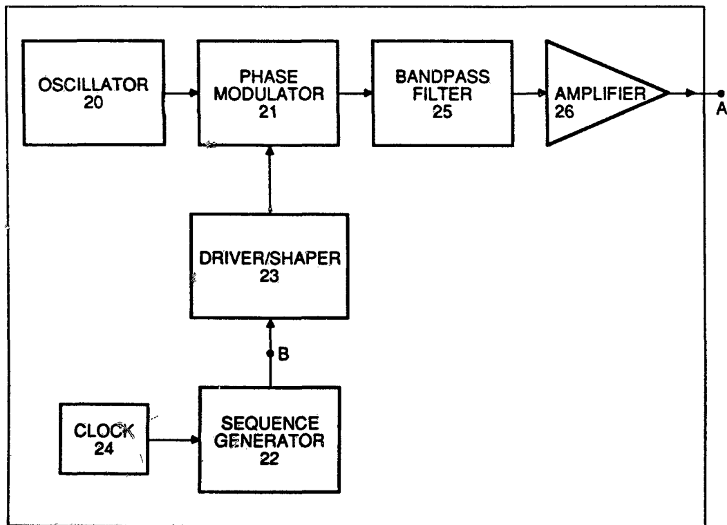
FIGURE 2. TRANSMITTER 10
