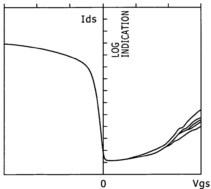
I_{ds} - V_{gs} CHARACTERISTIC OF P37
