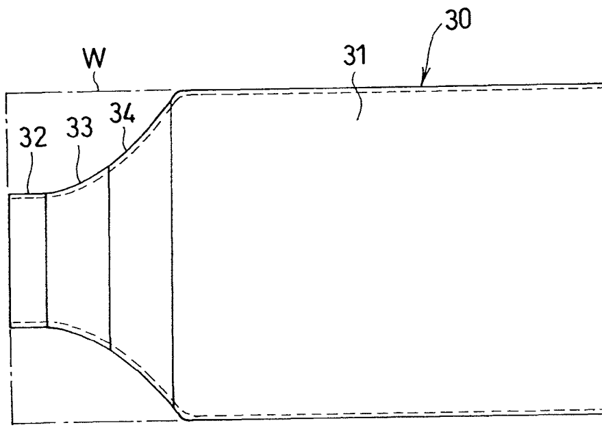
FIG. 11 PRIOR ART
