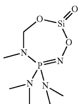
Phosphazene-silicate
