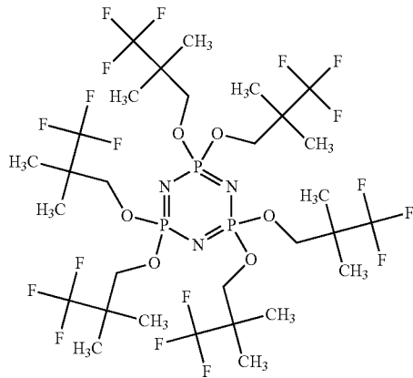
Hexakis(3,3,3-trifluoro-2,2-dimethylpropoxy)phosphazene
