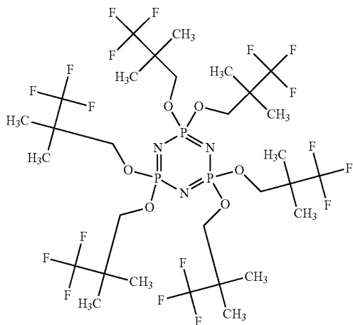
Hexakis(3,3,3-trifluoro-2,2-dimethylprooxy)phosphazene
