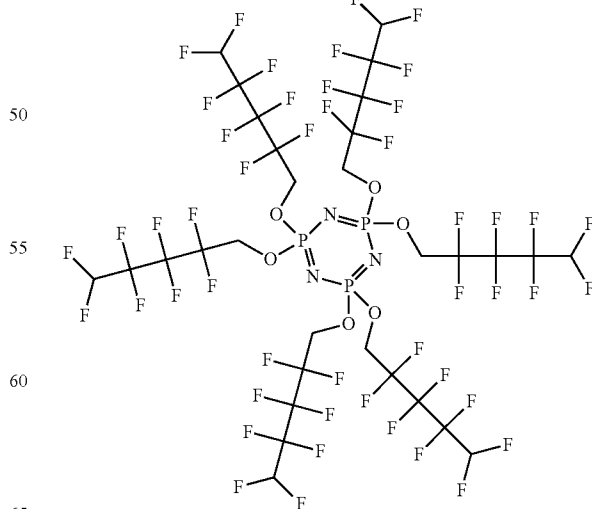
Hexakis(1H,1H,5H-octafluoropentoxy)phosphazene
