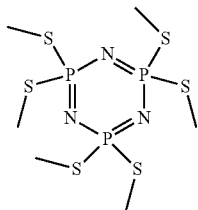
2,2,4,4,6,6-hexakis-methylsulfanyl-2λ5,4λ5,6λ5-cyclotriphosphazene
