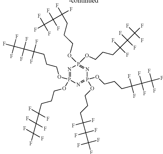
Hexakis(4,4,5,5,6,6,6-heptafluorohexoxy)phosphazene
