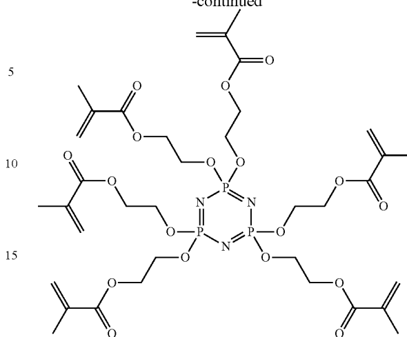
hexa(methacryloyloxy)cyclotriphosphazene
