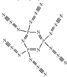
hexaazido cyclotriphosphazene
