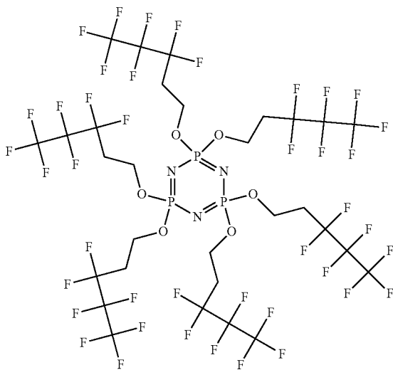
Hexakis (1H,1H,2H,2H-heptafluoropentoxy)phosphazene
