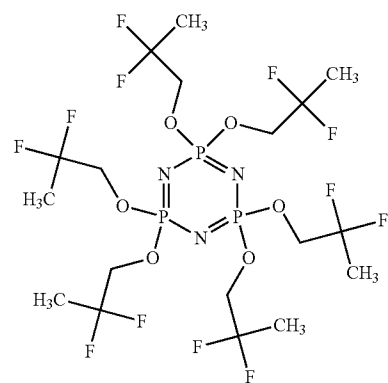
Hexakis(2,2-difluoropropoxy)phosphazene
