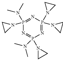
1,3,5,2,4,6-Triazatriphosphorine,2,2,4,4,6,6-hexahydro-4,6-bis(dimethylamino)-2,2,4,6-tetrakis(1-aziridinyl)-(CAS No. 3776-20-3)
