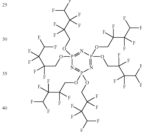
Hexakis(1H,1H,4H-perfluorobutoxy)phosphazene
