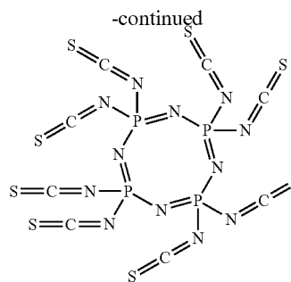
2,2,4,4,6,6,8,8-octaisothiocyanato-1,3,5,7-tetraza-2λ5,4λ5,6λ5,8λ5-tetraphosphacycloocta-1,3,5,7-tetraene
