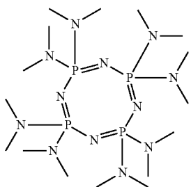
2,2,4,4,6,6,8,8-Octakis(dimethylamino)-1,3,5,7,2,4,6,8-tetrazatetraphosphocine
