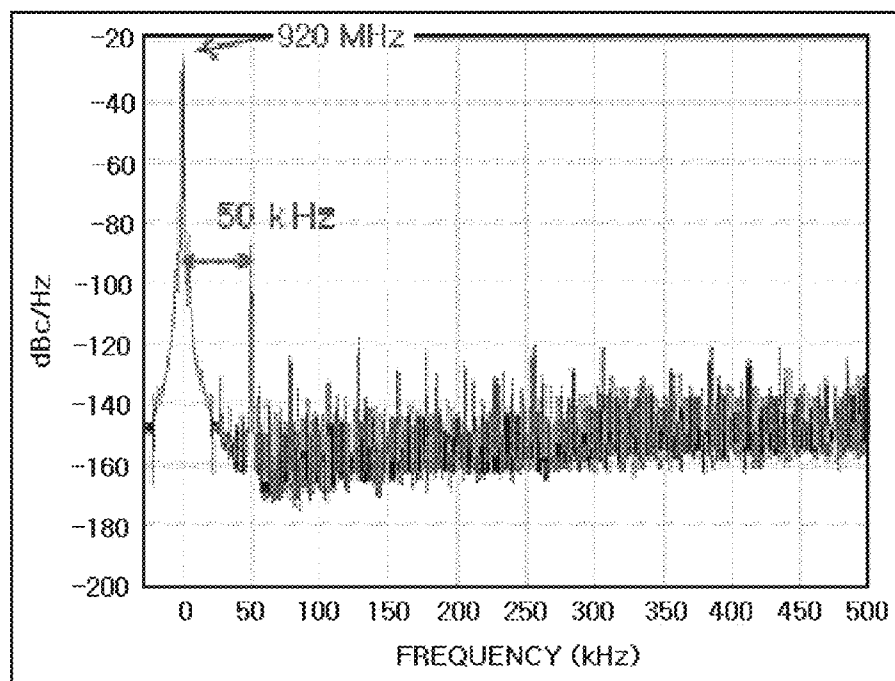
PLL OUTPUT SPECTRUM
