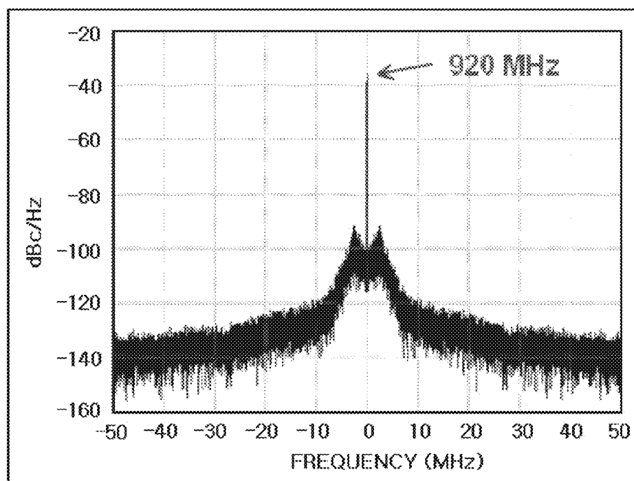
OUTPUT SPECTRUM OF DCO
