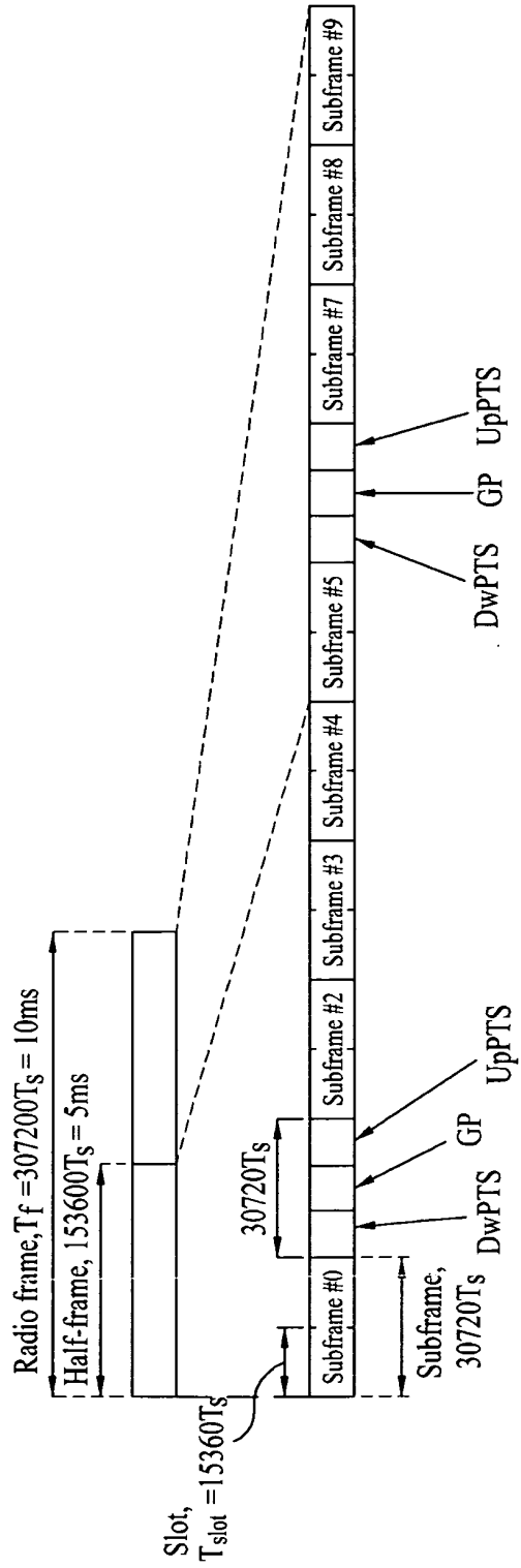
(b) Frame Structure Type 2
