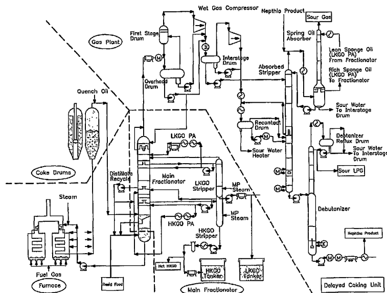
DCU and Light Ends Processing Units
