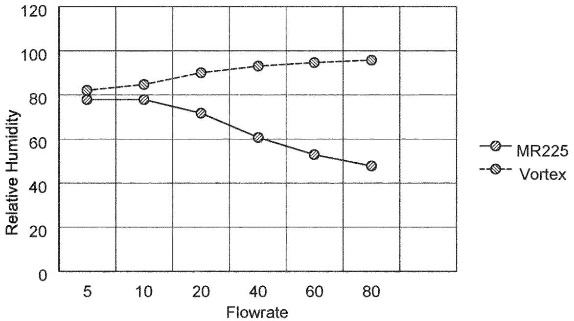
MR810 Humidity Output with MR225 and Vortex chambers
