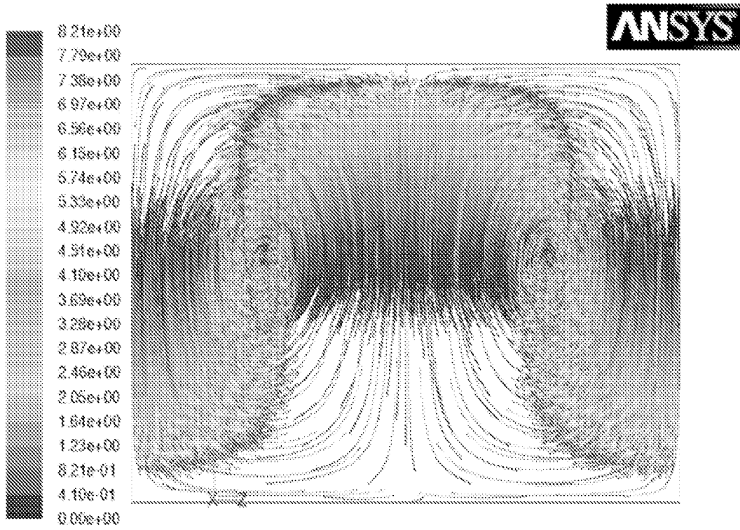
Particle Traces Colored by Particle Residence Time (s)
