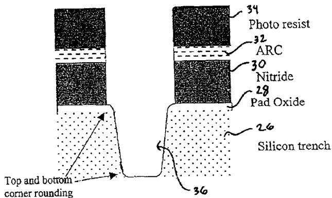
Post-etch diagram
