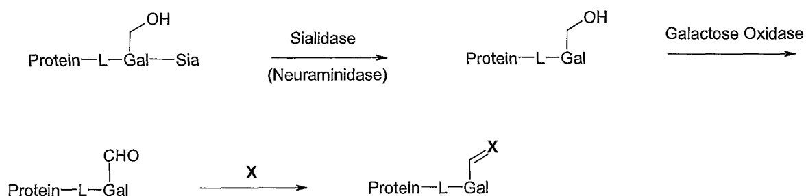
Reaction scheme 1
