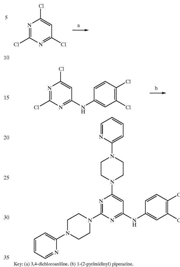
Scheme 5. Synthesis of the Compound of Example 43.
