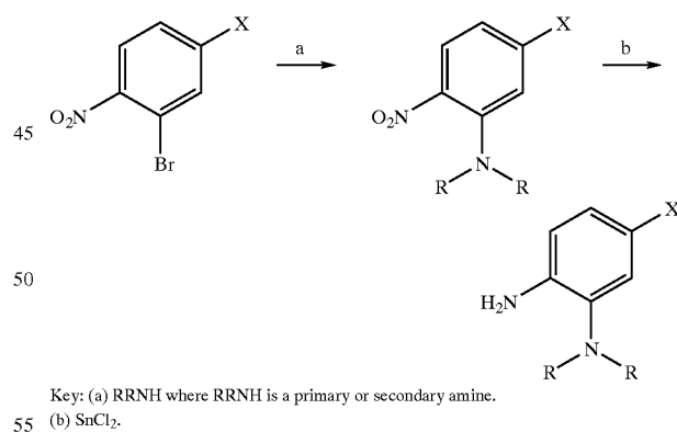
Scheme 6. Synthesis of Substituted 2-Aminoanilines.
