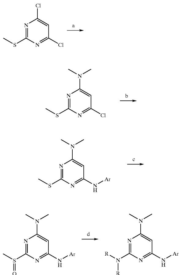
Scheme 3. Alternate Synthesis of Substituted 2,4,6-Triaminopyrimidines.
