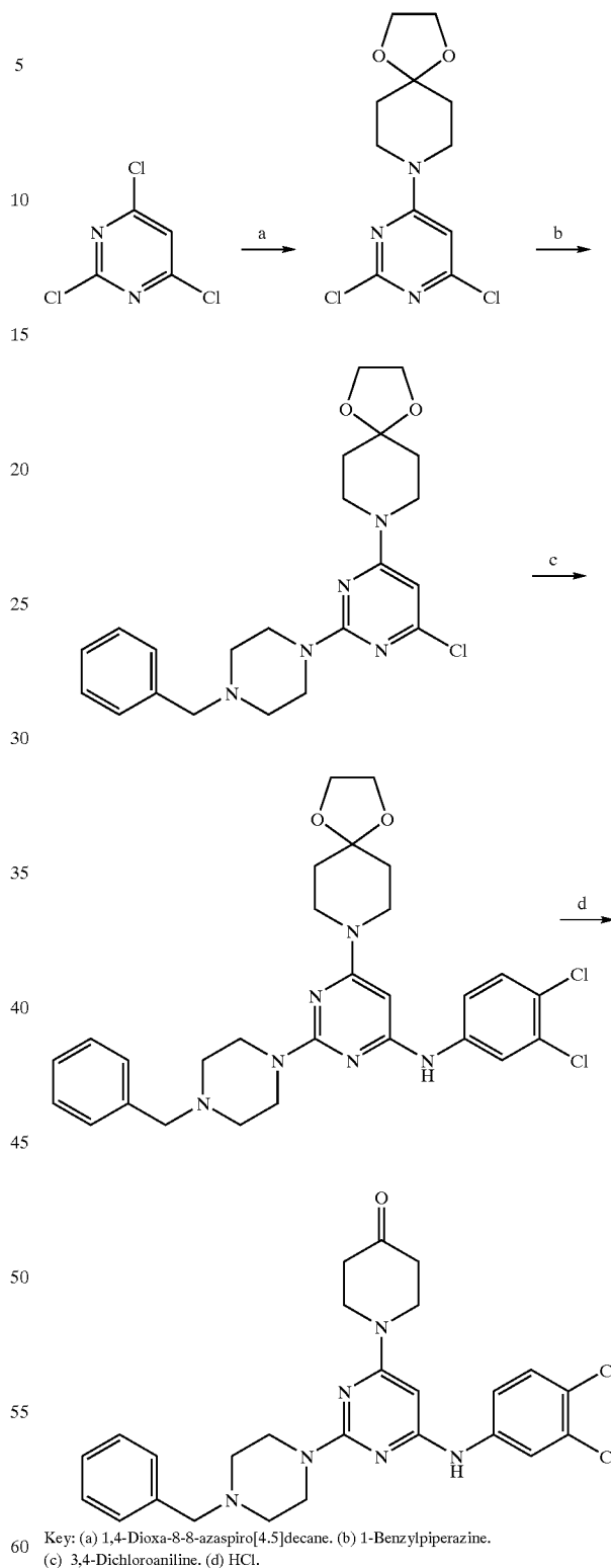
Scheme 2. Synthesis of the Compound of Example 53.
