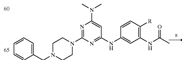
Scheme 7. Synthesis of the Compounds of Example 33 and 40.
