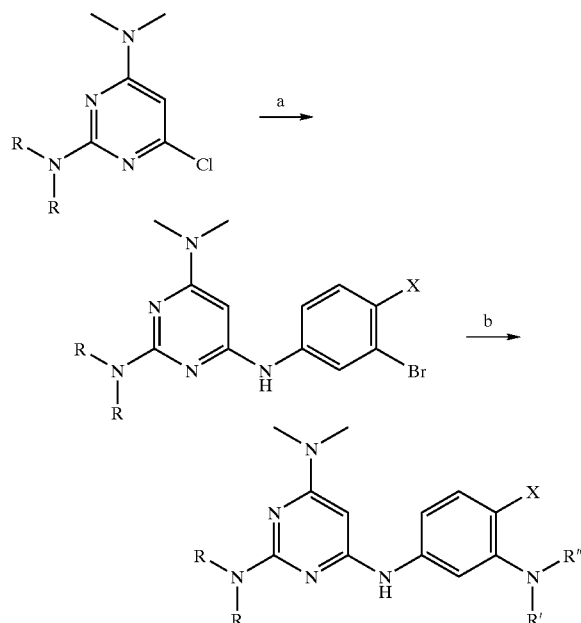
Scheme 8. Synthesis of the Compounds of Examples 26, 49 and 50.
