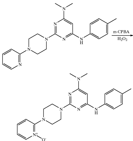
Scheme 4. Synthesis of the Compound of Example 46.
