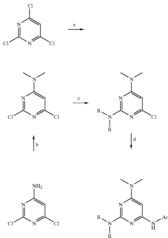
Scheme 1. Synthesis of Substituted 2,4,6-Triamino-pyrimidines.
