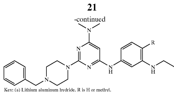
Scheme 8. Synthesis of the Compounds of Examples 26, 49 and 50.
