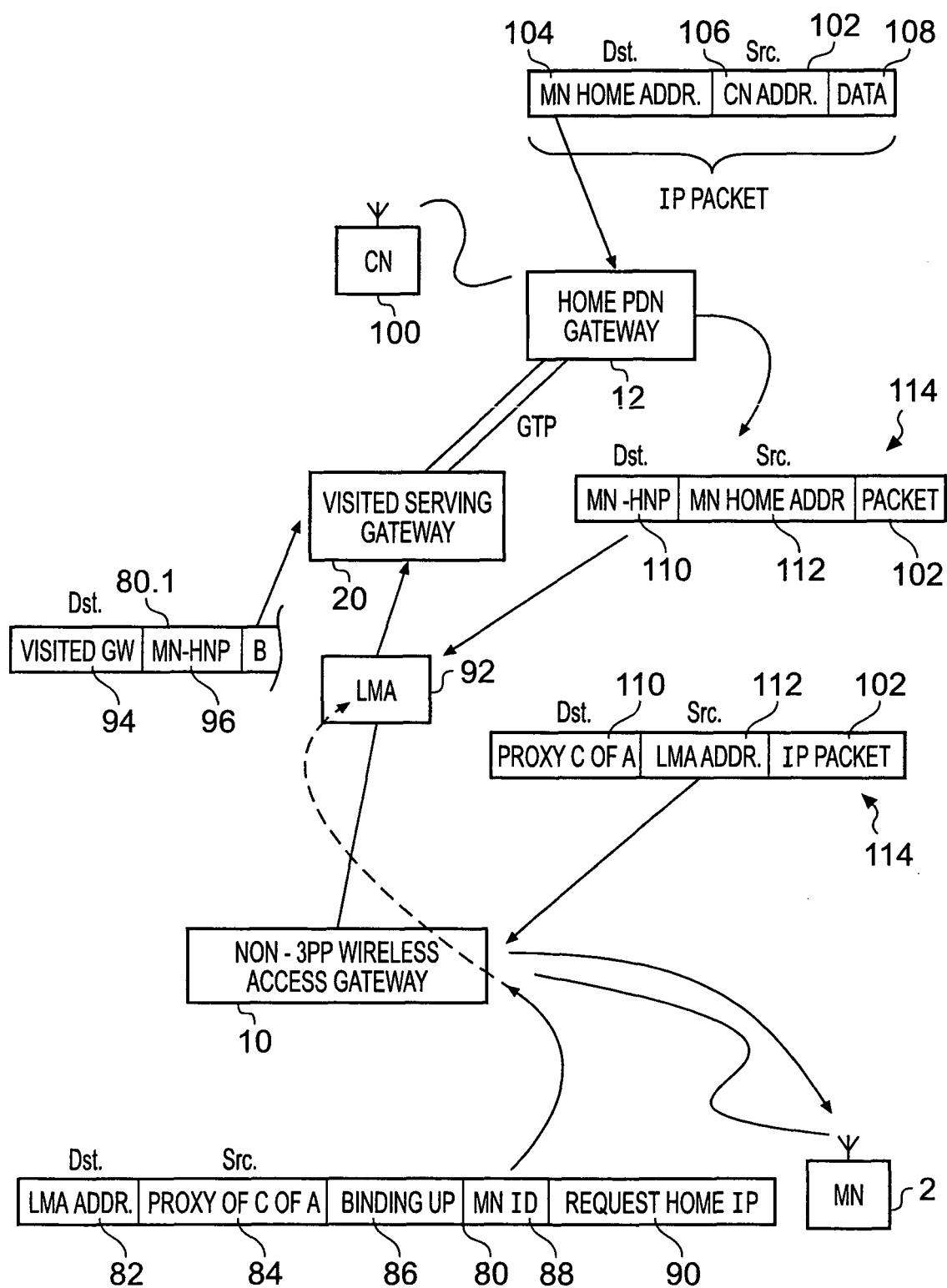
FIG. 6: PMIP Address Management
