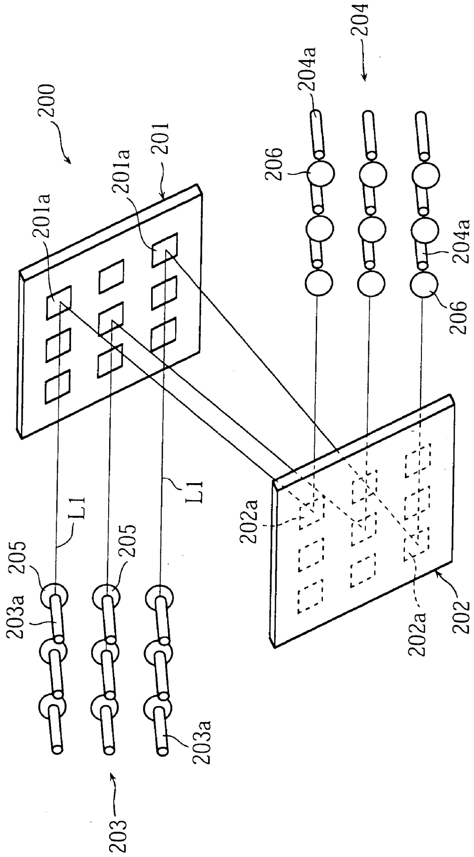
FIG. 39 PRIOR ART
