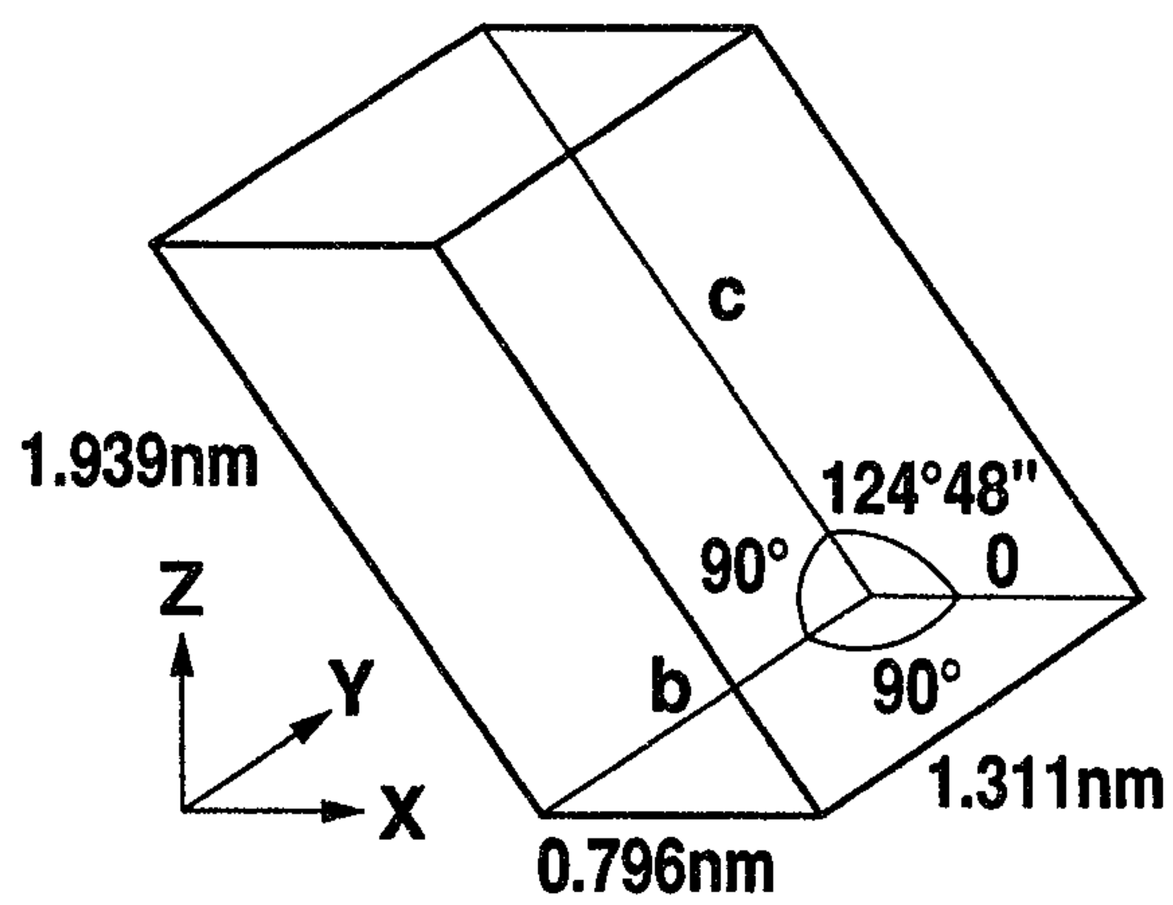
UNIT CELL OF POLYETHYLENE OXIDE CRYSTAL
