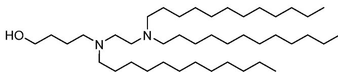
(Compound 20-22)
