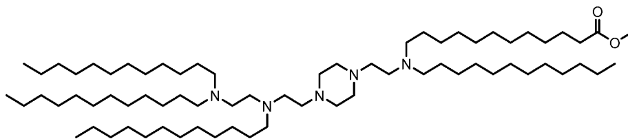
(Compound 15),
