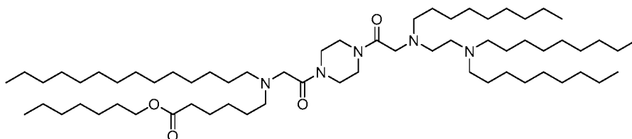
(Compound 91),
