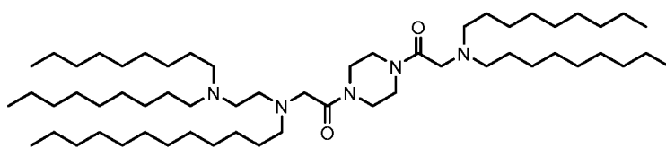
(Compound 5),
