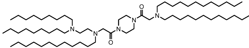
(Compound 9),
