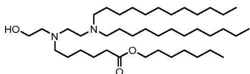
(Compound 20-7),
