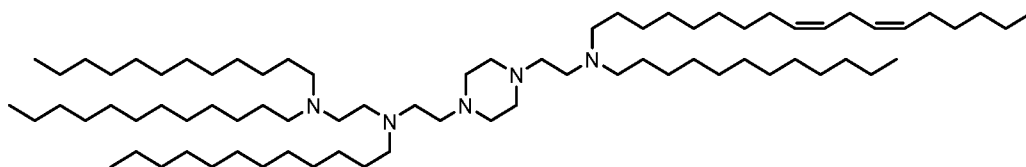
(Compound 27),
