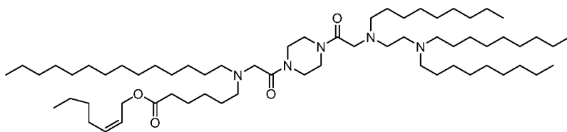
(Compound 108), and
