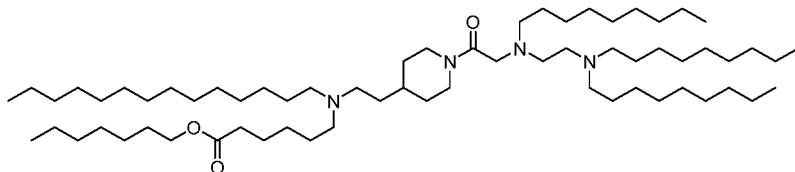
(Compound 94),
