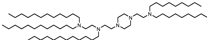
(Compound 23),
