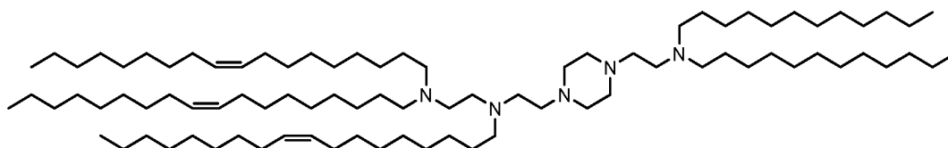
(Compound 33), and
