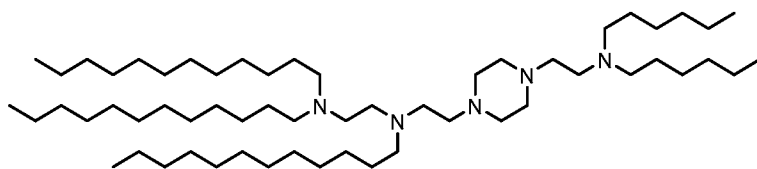
(Compound 21),
