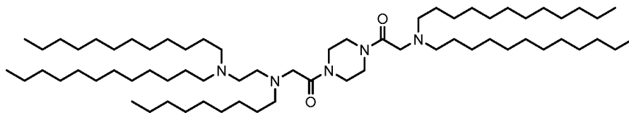
(Compound 9),
