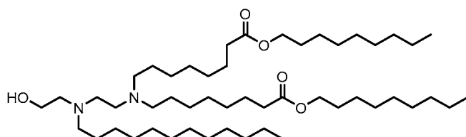
(Compound 20-10).
