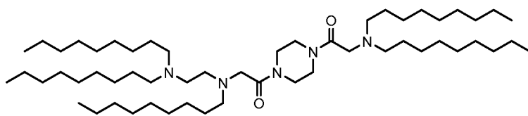
(Compound 4),
