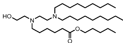
(Compound 20-6),
