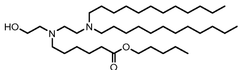
(Compound 20-3),
