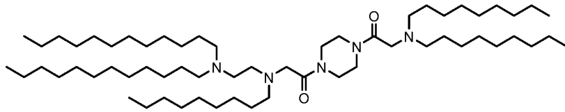
(Compound 5),
