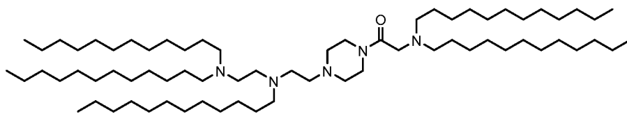
(Compound 3),
