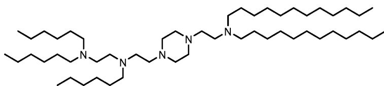
(Compound 17),
