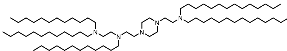
(Compound 26),
