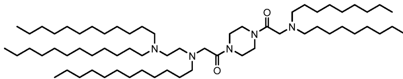
(Compound 7),
