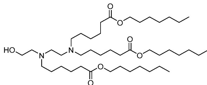
(Compound 20-5)
