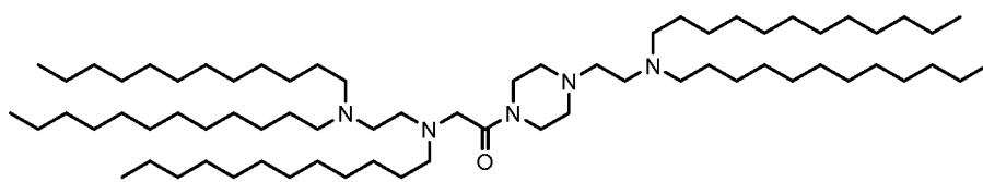
(Compound 2),
