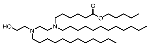
(Compound 20-2),
