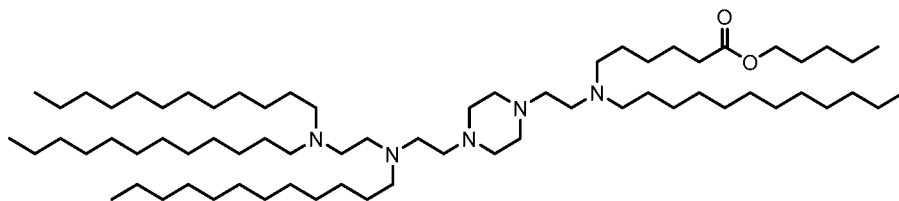
(Compound 12),
