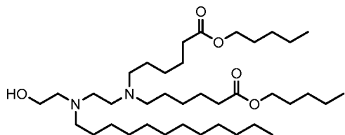
(Compound 20-4),
