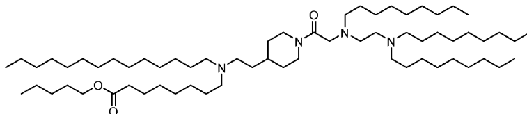
(Compound 93),
