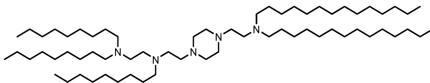
(Compound 20),
