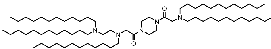
(Compound 11),
