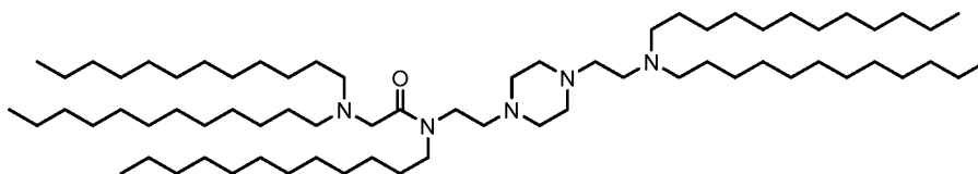
(Compound 1),
