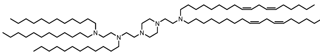
(Compound 29),
