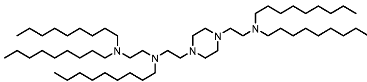
(Compound 18),
