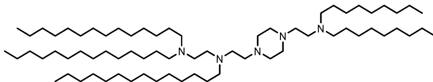
(Compound 30),
