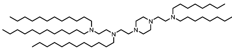
(Compound 22),
