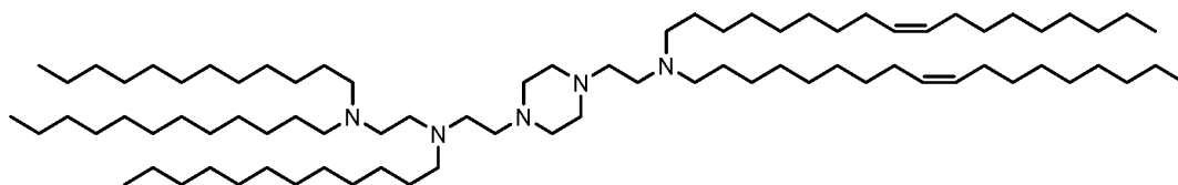
(Compound 28),
