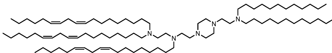
(Compound 34).
