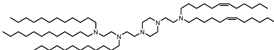
(Compound 25),
