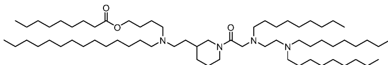
(Compound 95),
