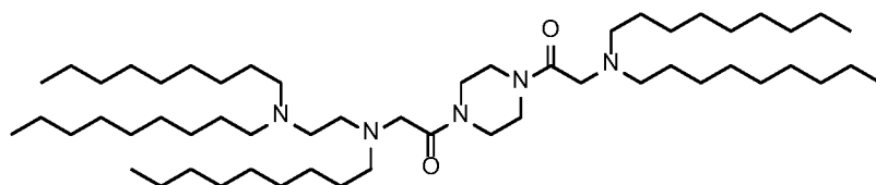
(Compound 4)
