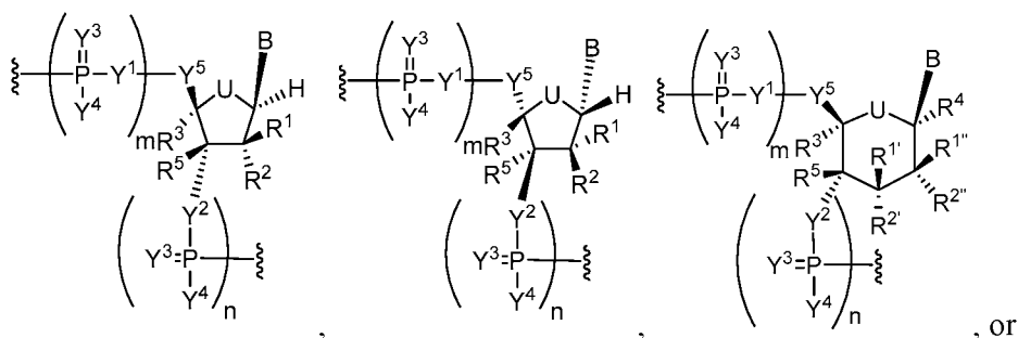
Formula VI
