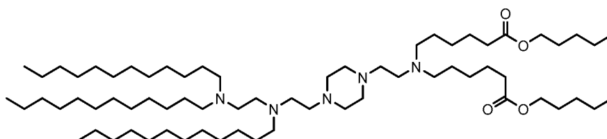
(Compound 14),
