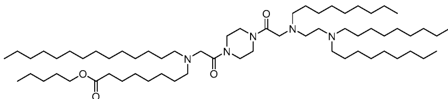
(Compound 90),
