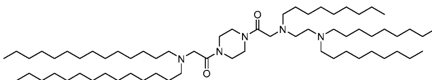
(Compound 50),
