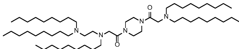
(Compound 4)
