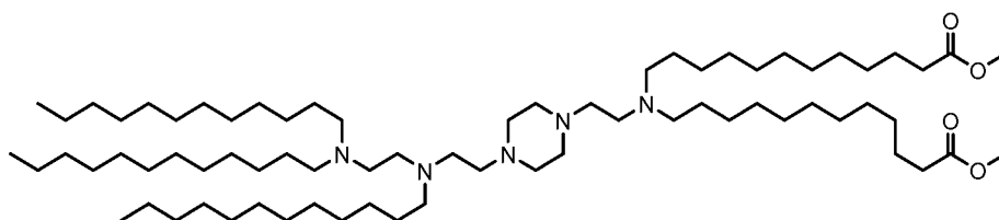
(Compound 16),
