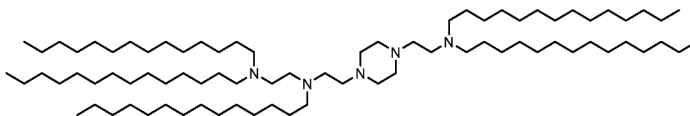
(Compound 32),
