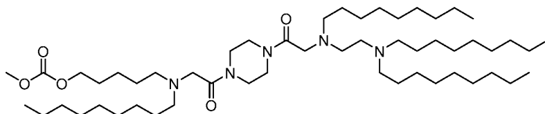
(Compound 109).
