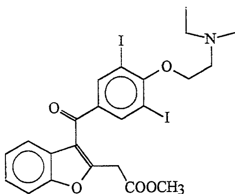
Compound A
