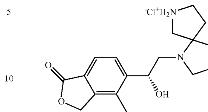
5-((1R)-1-Hydroxy-2-(1,7-diazaspiro[4.4]nonan-1-yl)ethyl)-4-methylisobenzofuran-1(3H)-one hydrochloride
