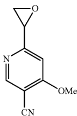
4-Methoxy-6-(oxiran-2-yl)pyridine-3-carbonitrile
