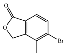
5-Bromo-4-Methyl-2-benzofuran-1(3H)-one
