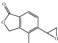
4-Methyl-5-oxiran-2-yl-2-benzofuran-1(3H)-one
