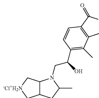
5-((1R)-1-Hydroxy-2-(2-methylhexahydropyrrolo[3,4-b]pyrrol-1(2H)-yl)ethyl)-4-methylisobenzofuran-1(3H)-one hydrochloride
