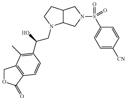
4-(1-((R)-2-Hydroxy-2-(4-methyl-1-oxo-1,3-dihydroisobenzofuran-5-yl)ethyl)hexahydropyrrolo[3,4-b]pyrrol-5(1H)-yl)sulfonyl)benzonitrile
