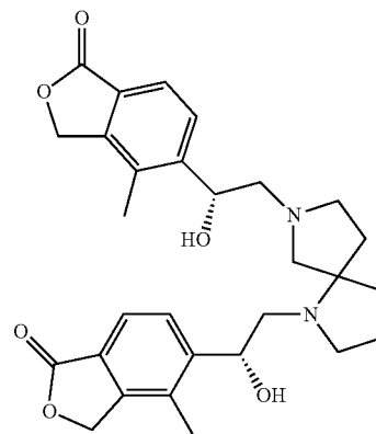
5,5'-(1R,1'R)-2,2'-(1,7-Diazaspiro[4.4]nonane-1,7-diyl)bis(1-hydroxyethane-2,1-diyl)bis(4-methylisobenzofuran-1(3H)-one)
