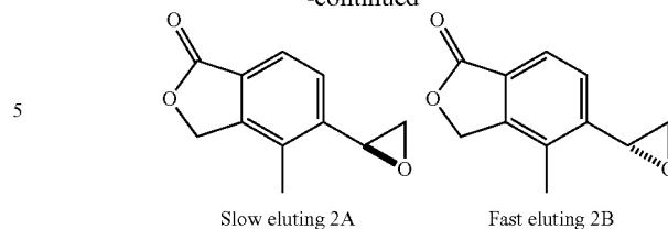
2A: 4-Methyl-5-[(2S)-oxiran-2-yl]-2-benzofuran-1(3H)-one
