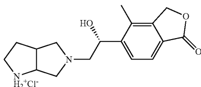
5-((1R)-2-(Hexahydropyrrolo[3,4-b]pyrrol-5(1H)-yl)-1-hydroxyethyl)-4-methylisobenzofuran-1(3H)-one hydrochloride
