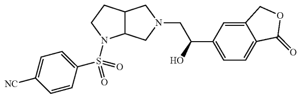
4-(5-((R)-2-Hydroxy-2-(1-oxo-1,3-dihydroisobenzofuran-5-yl)ethyl)hexahydropyrrolo[3,4-b]pyrrol-1(2H)-yl)sulfonyl)benzonitrile
